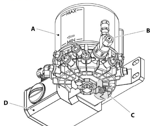
Lubrication pump
