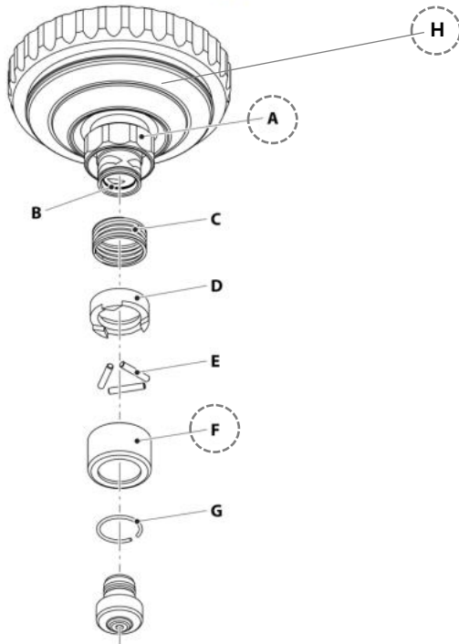
Disassembled nozzle quick-release coupling
